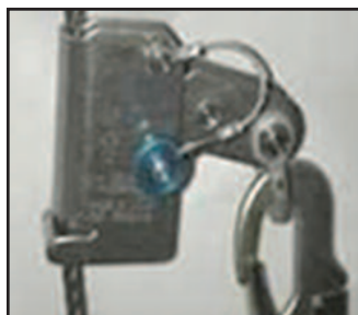
6. Check locking action by pulling down on rope grab handle.
