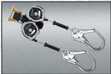
RD-HNY8CT - 8' Wire Y-Retractable Lanyard with 3,600 lb Gates Top and Bottom. Includes two steel rebar hooks.
