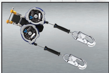
RD-HNY8 - 8' Wire Retractable Lanyard with 3,600 lb Gates Top and Bottom. Includes two snap hooks (96595).
