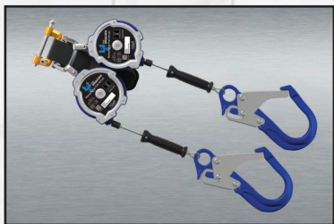
RD-HNY8CA - 8' Wire Y-Retractable Lanyard with 3,600 lb Gates Top and Bottom. Includes two large aluminum rebar hooks.
